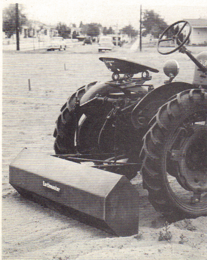
Earthmaster Scraper No. 165 — 5 feet wide — Hydraulic depth control
